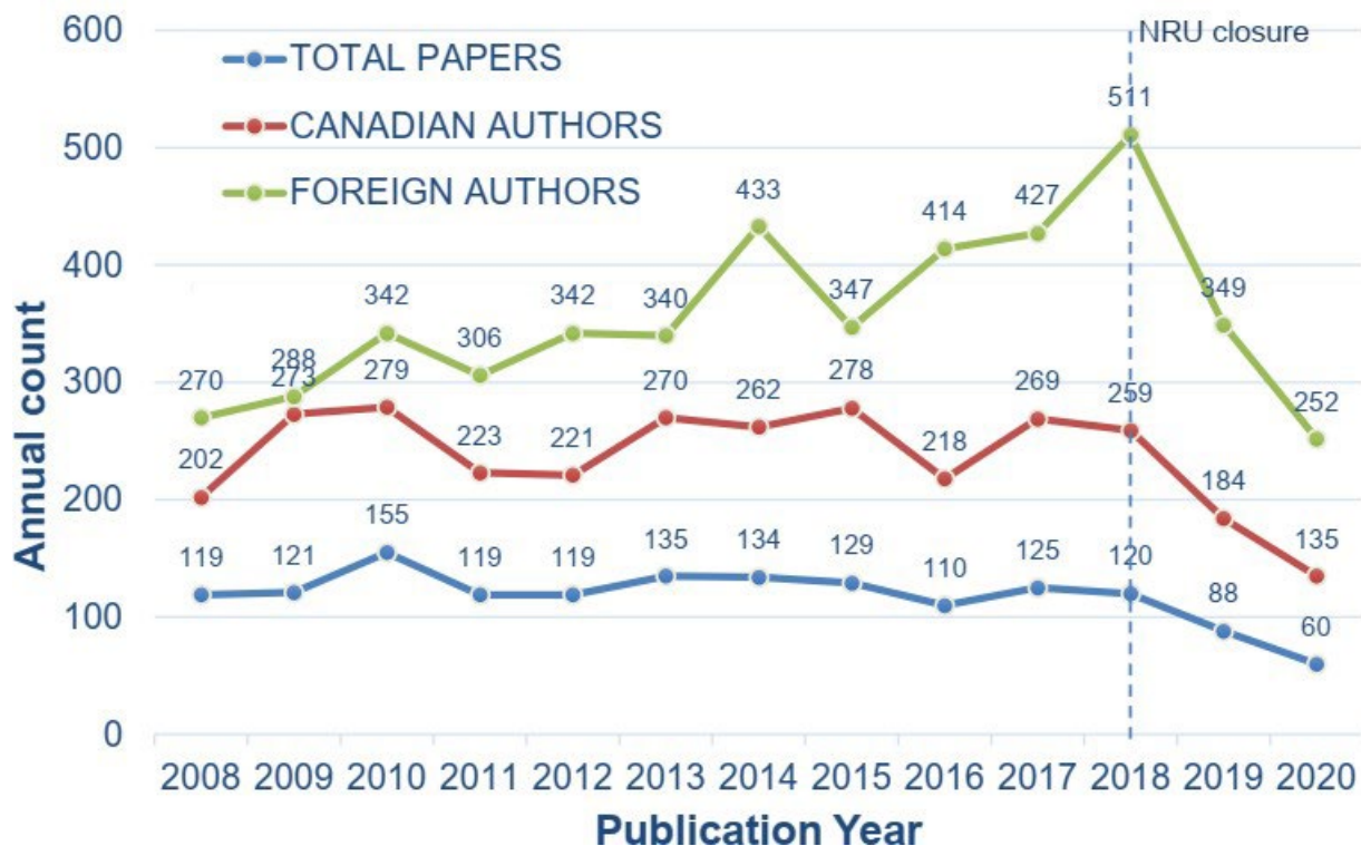
Figure 8 Annual publication count of neutron beam papers with at least one Canadian author in the Web of Science database using methods described in footnote 19. The NRU reactor, the source of neutrons for the CNBC, closed in 2018. Source: Prof. Thad Harroun.
