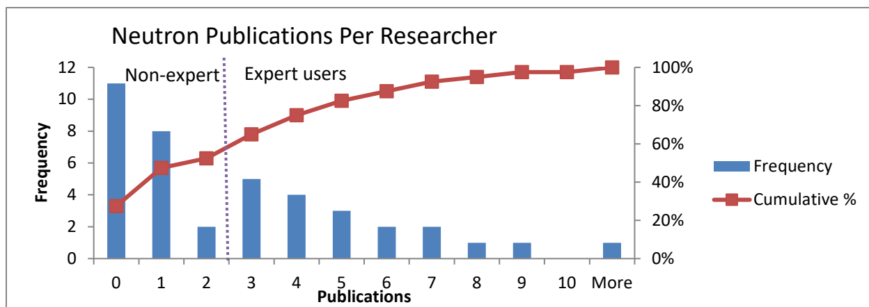
Figure 5. Histogram of the frequency of neutron beam publications in the two years following the closure of the CNBC among 40 neutron beam users, primarily Canadian faculty researchers. Source: CINS-CNI 2020 survey
